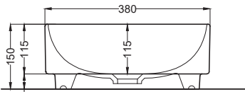
SIDE
