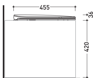
art. AS117G - AS117RG vista laterale / lateral view
