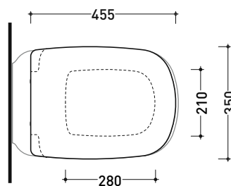
art. MN118 / MN118S vista zenitale / zenital view
